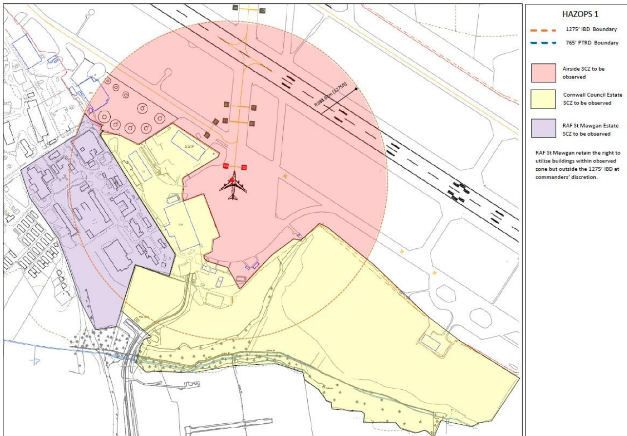
Figure 13: Spaceport Side Layout with Security & SCZ Boundaries (detailing 1275ft SCZ)
